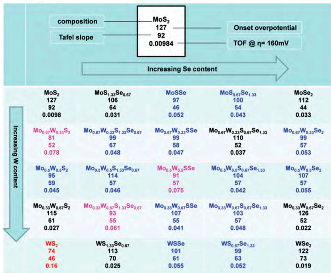
Figure 10. Summarizing the onset overpotential, Tafel slope and TOF @ \eta = 160\text{ mV} of different compositions. The red color labels compositions with TOF > 0.1\text{ s}^{-1} ; the magenta color labels compositions with 0.06 < \text{TOF} < 0.1\text{ s}^{-1} ; the blue color labels compositions with 0.04 < \text{TOF} < 0.06\text{ s}^{-1} . Adapted with permission from Reference [139], copyright (2016), Wiley-VCH.
