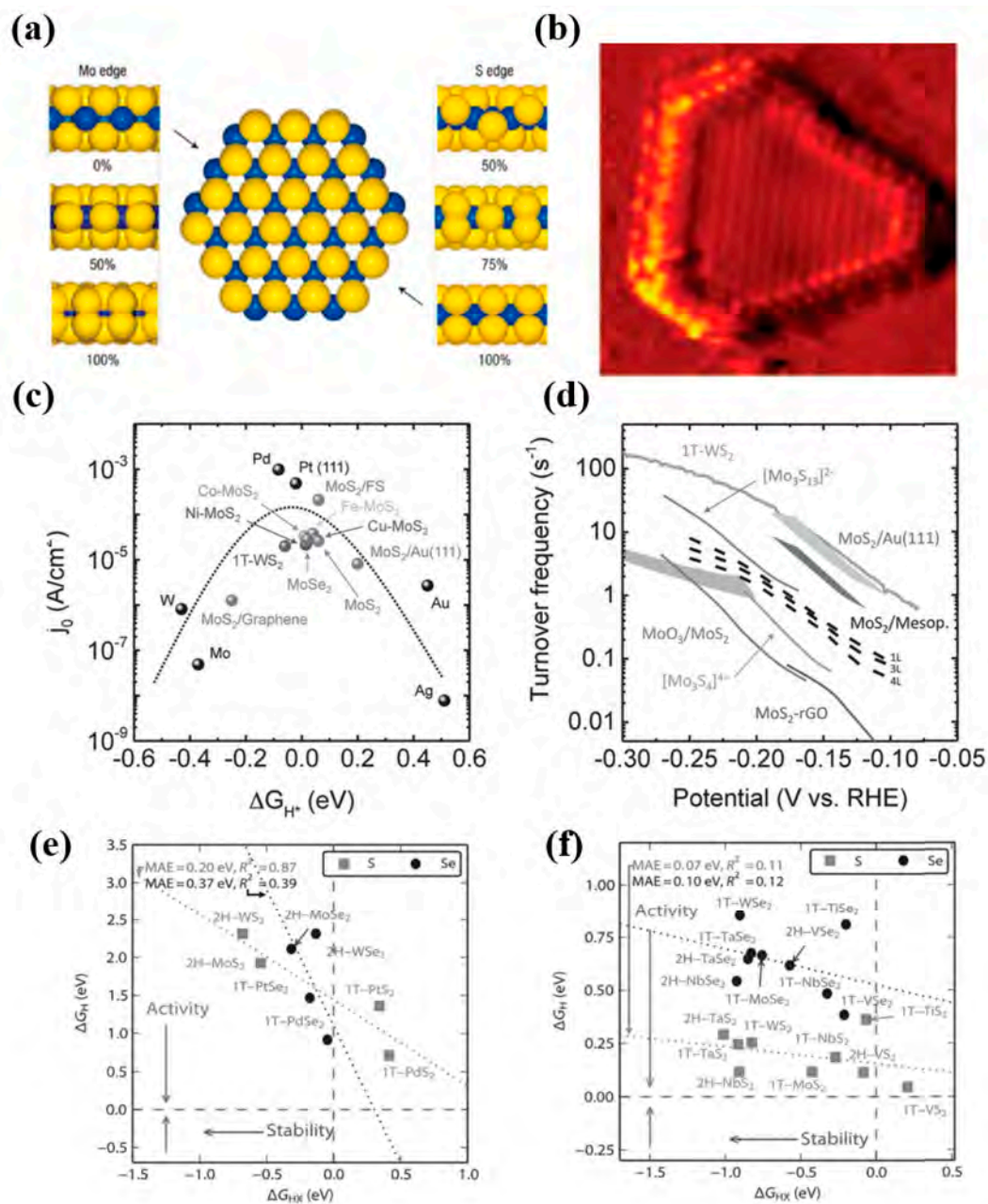
Figure 3. (a) Molecular model of a platelet exposing both Mo and S-edges from top and side view. Reprinted with permission from [79], copyright (2014), American Chemical Society. (b) STM on MoS 2 nanoplatelets on Au (111). Reprinted with permission from Reference [77], copyright (2007), American Association for the Advancement of Science. Thermodynamics of hydrogen adsorption on 2D transition metal dichalcogenides. (c) Sabatier “volcano” plot showing the exchange current density as a function of free energy of hydrogen adsorption of free-standing (FS) MoS 2 edges, MoS 2 edges on Au (111), MoS 2 edges on graphene, vertically grown Fe, Cu, Ni, Co-promoted MoS 2 edges, vertically grown MoS 2 edges, vertically grown MoSe 2 edges, 1T WS 2 basal plane and compared with various metals. (d) Evolution of turnover frequency of several catalysts based on transition-metal chalcogenides with overpotential. (e,f) Plots of \Delta G_{H^*} : the free energy of hydrogen adsorption as function of \Delta G_{HX} (X = S or Se): the HX adsorption free energy. (e,f) The evolution is displayed for metallic TMDs (e) and semiconducting TMDs (f). In general the stronger binding of X ( \Delta G_{HX} < 0 ), the higher stability of TMDs, the lower the reactivity of TMDs ( \Delta G_{H^*} > 0 ), the weaker the hydrogen binding. Reprinted with permission from Reference [23], copyright (2016), Wiley-VCH.
