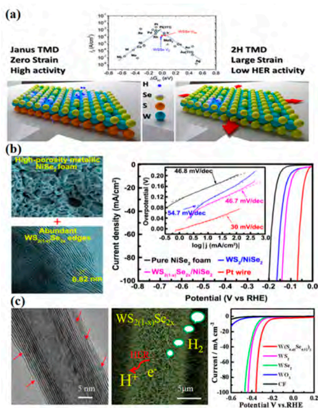
Figure 7. (a) Schematic for WS 2 Se with \Delta G_{\text{H}} “volcano” plot, the illustration shows that strain free Janus TMDs possess better HER activities. Reprinted with permission from [125], copyright (2018), American Chemical Society. (b) TEM of WS 2(1-x)Se 2x particles with a 3D porous metallic NiSe 2 foam and corresponding polarization curves recorded on WS 2(1-x)Se 2x /NiSe 2 foam. (c) TEM of WS 2(1-x)Se 2x nanotubes and corresponding polarization curves recorded on WS 2(1-x)Se 2x in comparison with WS 2 . Reprinted with permission from Reference [67], copyright (2014), American Chemical Society.
